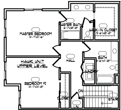
HAWK UNIT UPPER LEVEL
