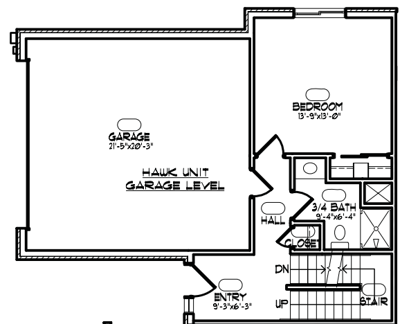
HAWK UNIT GARAGE LEVEL
