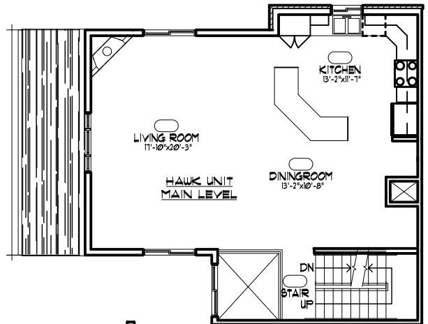
HAWK UNIT MAIN LEVEL
