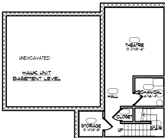
HAWK UNIT BASEMENT LEVEL
