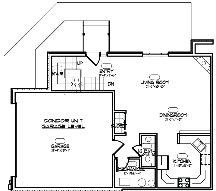
CONDOR UNIT NORTH GARAGE LEVEL
