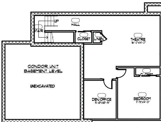
CONDOR UNIT NORTH BASEMENT LEVEL
